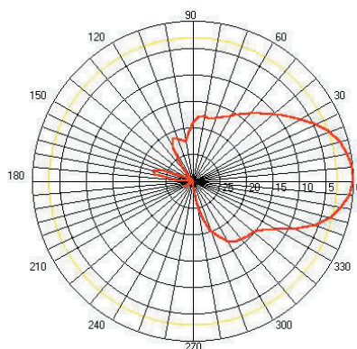
WIES24-14 E Plane
