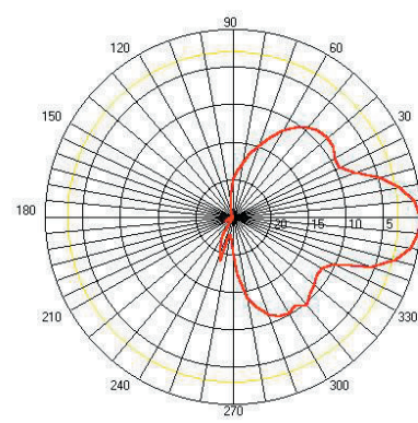
WIES24-14 H Plane
