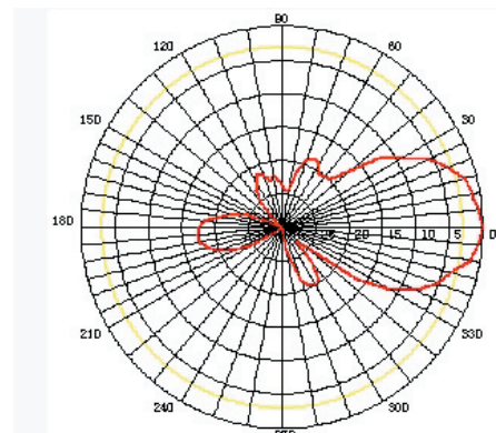
E Plane - Vertical
