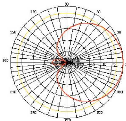
H Plane - Azimuth
