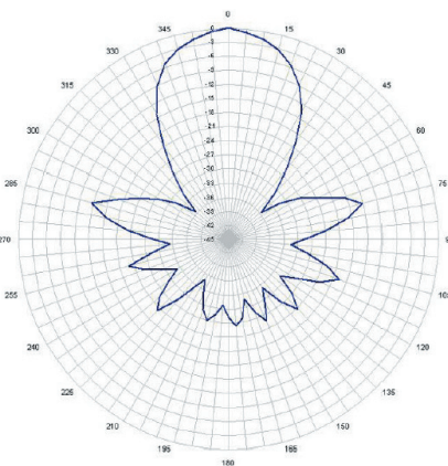
E Plane - Vertical
