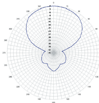
H Plane - Azimuth
